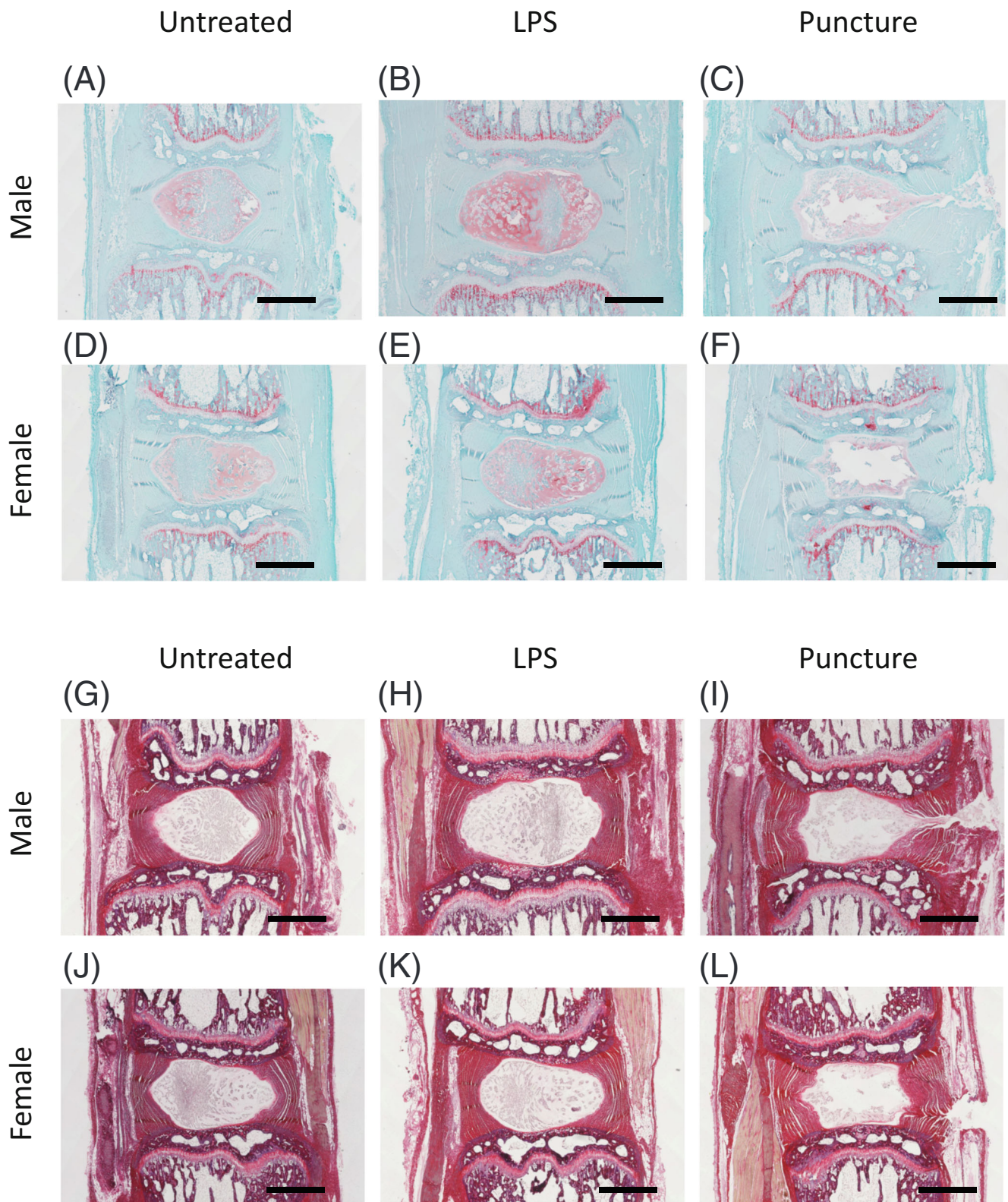
FIGURE 7 Safranin O with Fast Green staining of short-term male (A) untreated, (B) LPS, and (C) puncture and female (D) untreated, (E) LPS, and (F) puncture discs. Picrosirius Red staining of short-term male (G) untreated, (H) LPS, and (I) puncture and female (J) untreated, (K) LPS, and (L) puncture discs. Scale bar: 1 mm. LPS, lipopolysaccharide.
