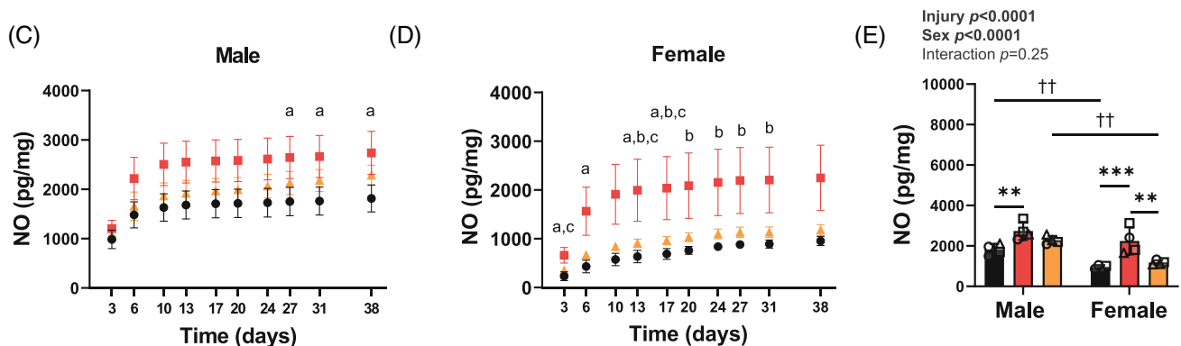
FIGURE 2 Cumulative short-term release of (A) HMGB1 and (B) NO into disc media * p < 0.05 (each symbol represents a different donor in each sex). Long-term release of NO into the media from (C) male and (D) female motion segments in each group. (E) Day 38 cumulative NO release ( N = 4 , each symbol represents a different donor in each sex). * p < 0.05 , ** p < 0.01 , *** p < 0.001 , **** p < 0.0001 , a p < 0.05 for untreated versus LPS, b p < 0.05 for untreated versus puncture, c p < 0.05 for LPS versus puncture, # p < 0.1 for post hoc between injury, and † p < 0.05 , †† p < 0.01 for post hoc between sex). LPS, lipopolysaccharide; NO, nitric oxide.
